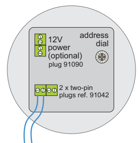
2c to lighting control module or shared/Dali bus
